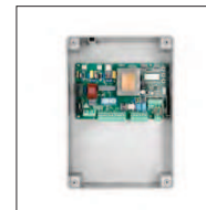
230 Vac control panel with built-in 433.92 Mhz 64-code receiver, integrated display and fixed slowing-down functions. (for full features see page 154)
